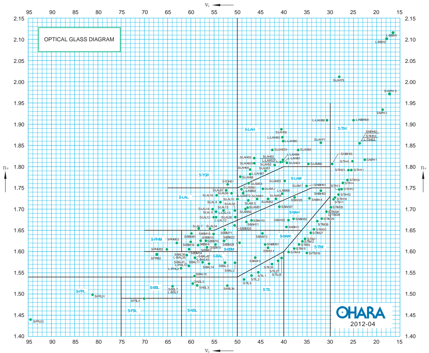
n_e - \nu_e Diagram
